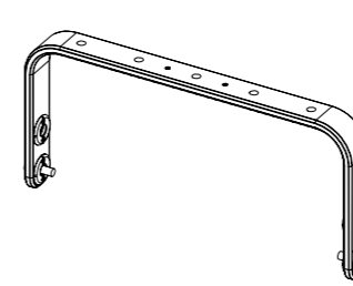
Horizontal mounting bracket VNU-HBRK365 bracket for ePS6-EN54 VNU-HBRK425 bracket for ePS8-EN54 VNU-HBRK535 bracket for ePS10-EN54 VNU-HBRK600 bracket for ePS12-EN54
