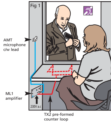
A typical counter loop system using components included the ML1/K kit
