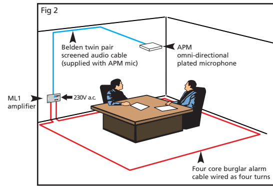
A typical 20m 2 small room system using an ML1 amplifier, an APM plated microphone and four core burglar alarm cable
