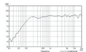
Frequency Response
